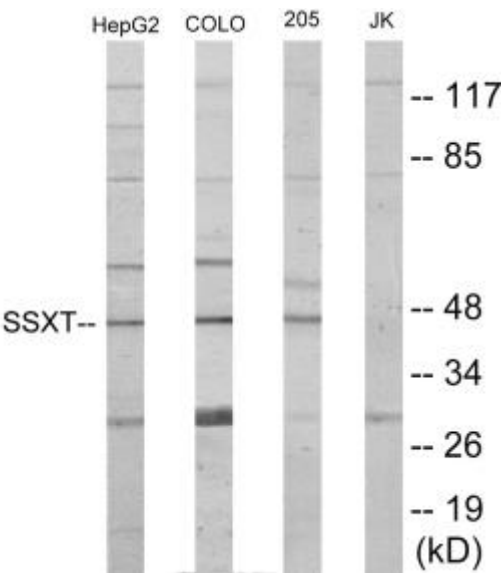
Figure 1. Anti-SSXT
