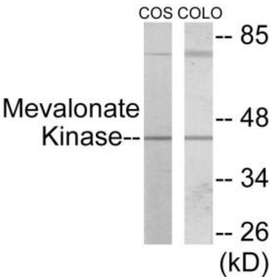
Figure 1. Anti-Mevalonate Kinase
